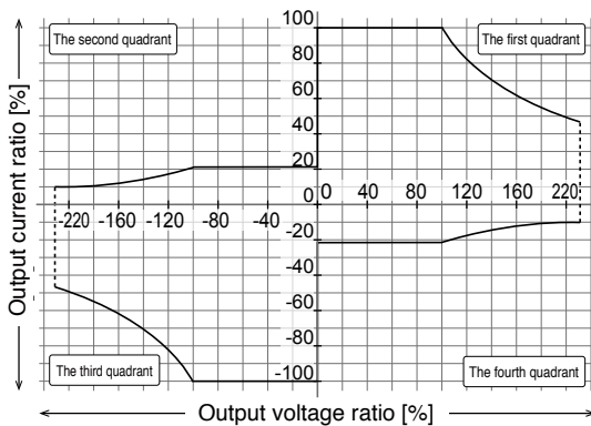
■ Output voltage ratio versus rated output current characteristics (DC mode)
