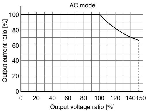
■ Output voltage ratio versus rated output current characteristics (AC mode)
