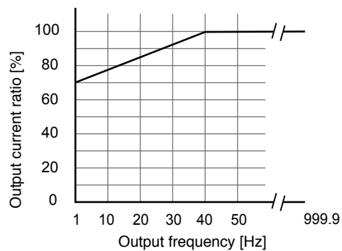
■ Output frequency versus rated output current characteristics
