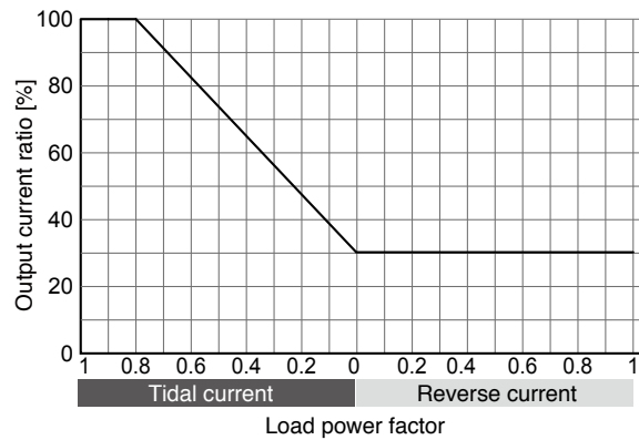
■ Load power factor versus rated output current characteristics
